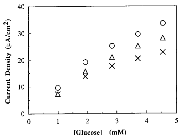
Figure 5 Calibration curves for poly(hydroquinone) glucose sensor at different working potentials. Sensor composition is graphite: PHQ: GOD = 1: 1: 0.5. (o) 400 mV; (Δ) 200 mV; and (x) 100 mV.
