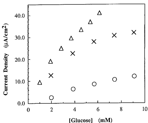
Figure 4 Calibration curves for poly(hydroquinone) glucose sensors. The weight ratio in the sensors are graphite: PHQ: GOD = (Δ) 1: 1: 0.5; (X) 1: 0.5: 0.25; (o) 1: 0.5: 0.1. The working potential is 400 mV versus SCE.
